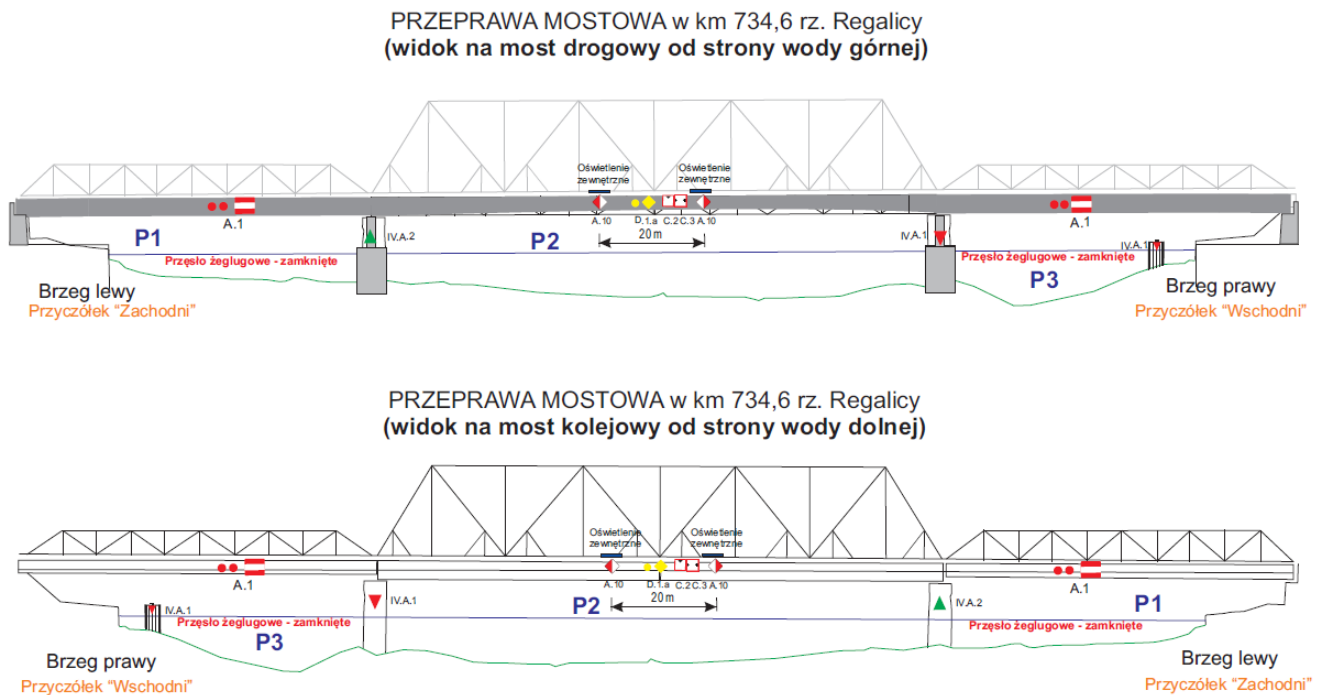
Fig.1 Shipping traffic under the middle bridge span
