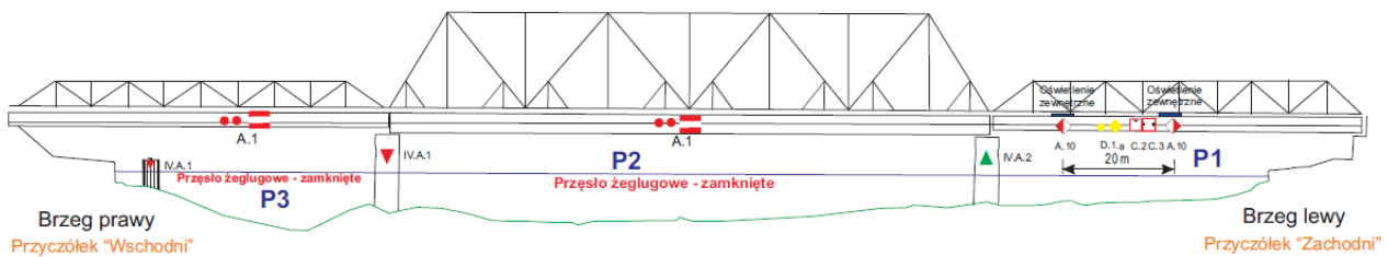
Fig.2 Shipping traffic under the western bridge span
